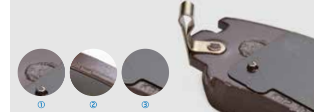
Figure 4. Counterfeit parts of the brake pads made with easily detachable shim; haphazard molding with thinner edges
